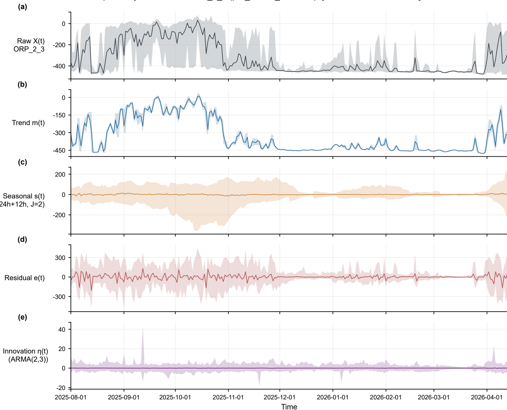
Full-span daily overview — ORP_2_3 (pre_anoxic_rear, min) [2025-08-01~2026-04-13]
